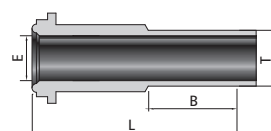
GFS Gland to Long Fractional Tube Butt Weld
