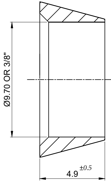
FRONT FERRULE
