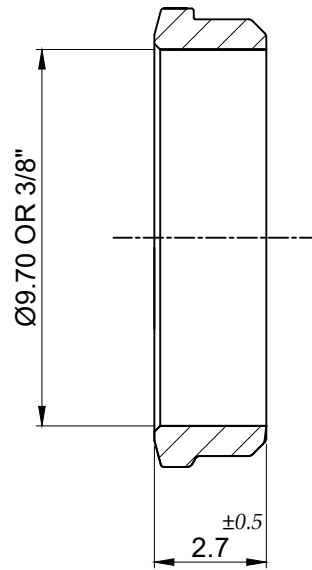
BACK FERRULE
