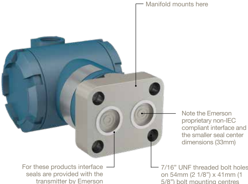
3051 DP transmitter, shown with the Emerson flange adapter removed.
