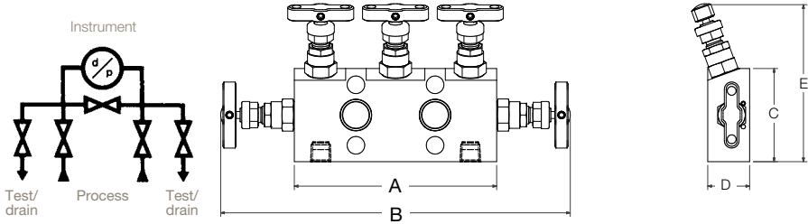
Example shown: 5-valve extruded direct mount manifold with Parker Superior Advantage fully integrated inverted A-LOK® tube fitting connections.
