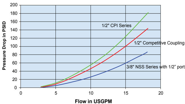
3/8" NSS vs 1/2" Instrumentation Coupler Pressure Drop vs Flow
