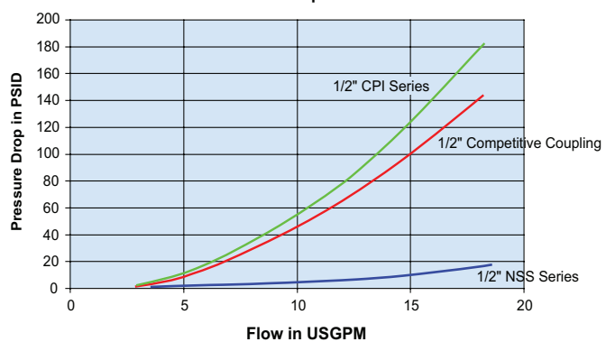
1/2" NSS vs 1/2" Instrumentation Coupler Pressure Drop vs Flow
