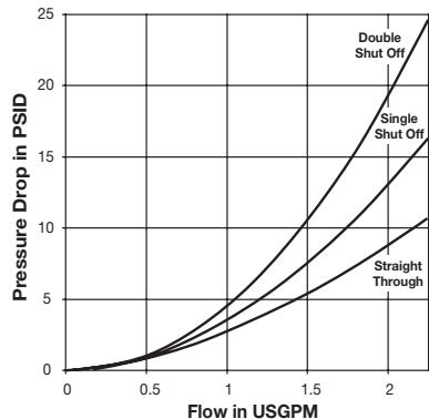
Spectrum Series (1/8") Test Fluid: Water
